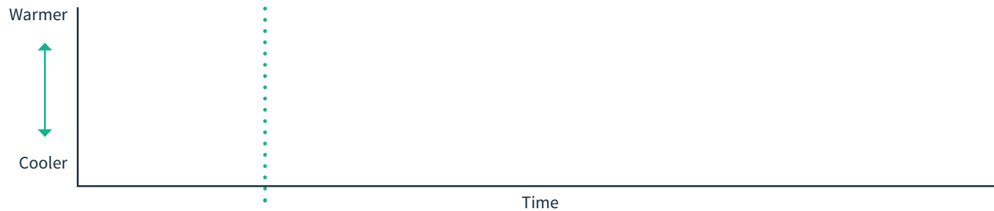
Temperature at the Earth surface
