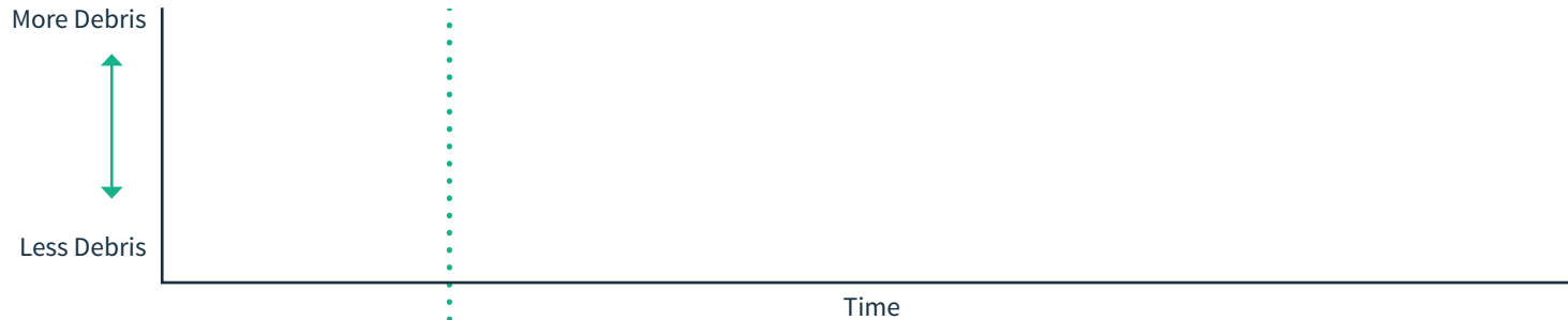
Amount of volcanic debris in atmosphere
