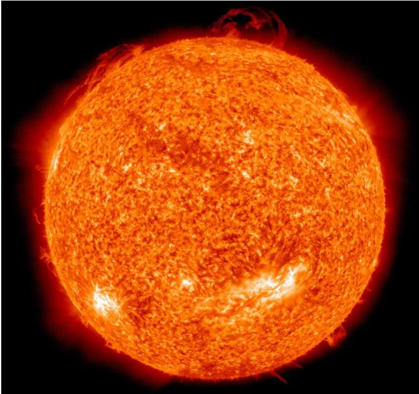
Ultraviolet View of the Sun – September 19, 2010
